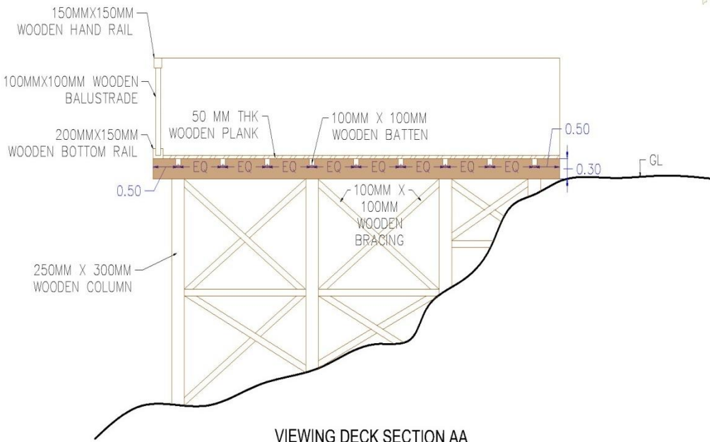
VIEWING DECK SECTION AA
