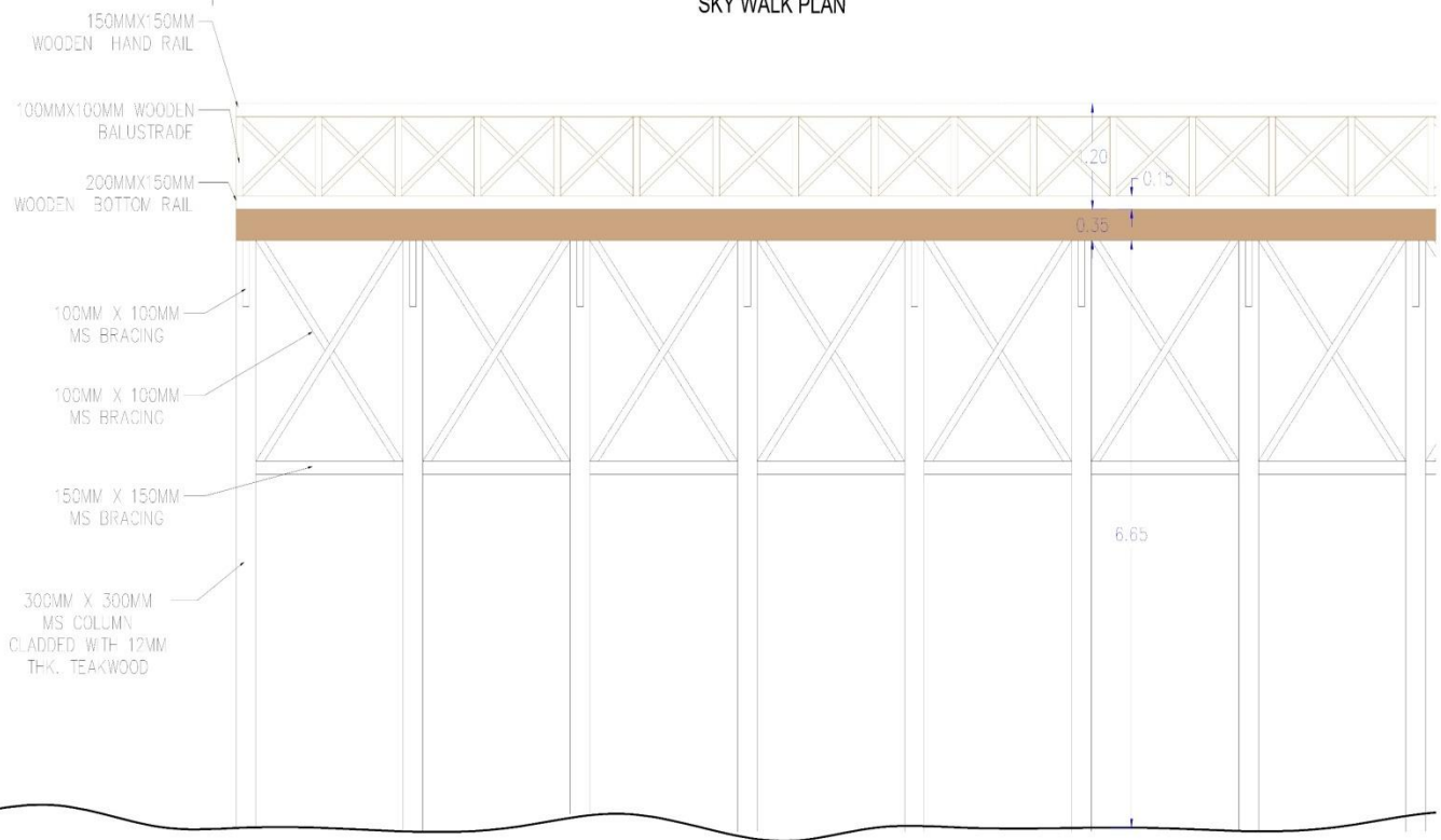
SKY WALK ELEVATION
