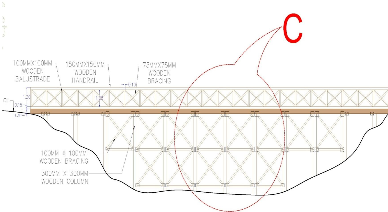
BRIDGE ELEVATION
